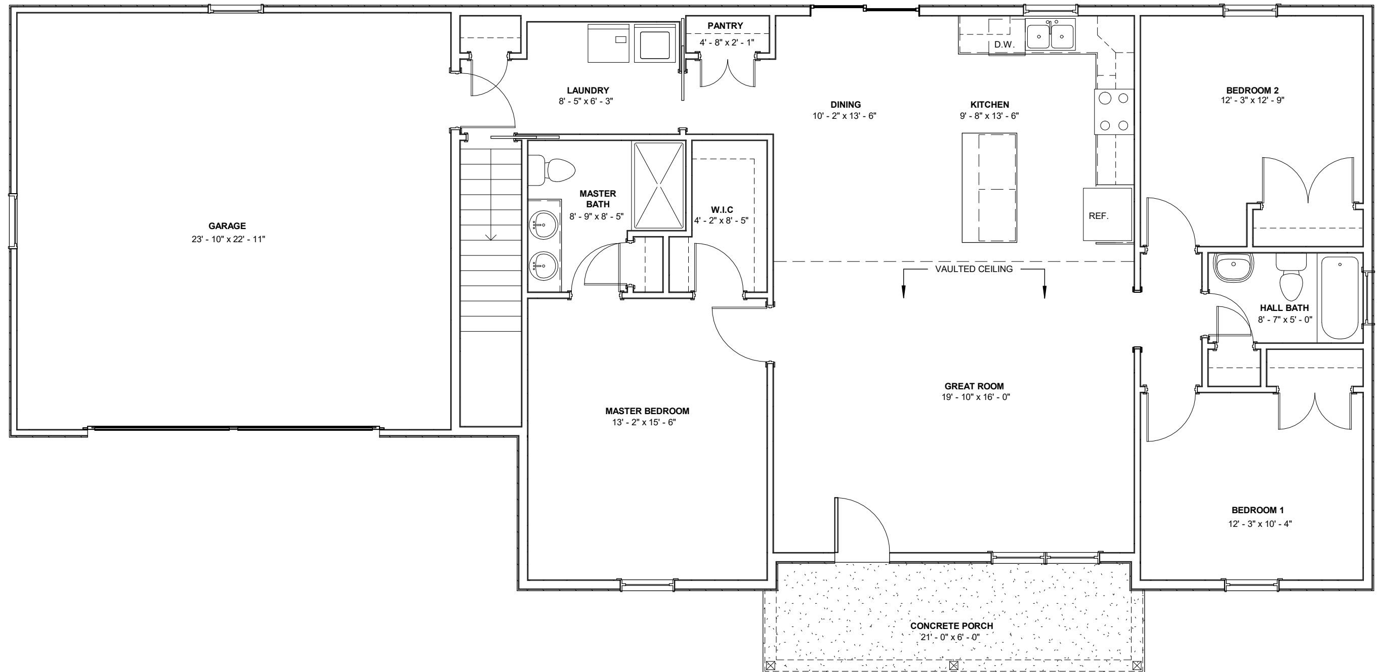
FIRST FLOOR SIMPLIFIED
